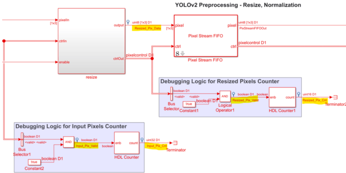
This figure shows the signals that are configured as test points in the DLHandshakeLogicDebug model.
